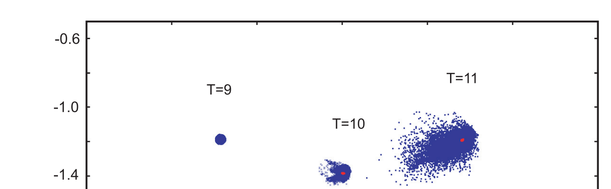
The dynamics of gaseous (red) and solid (blue) model particles fixed in the moment T=9 in the marked individual high-density area. The collapsing clump of gas moves as a volume of fixed compound, while the solids are scattered around due to the gradient of gravitational potential.
