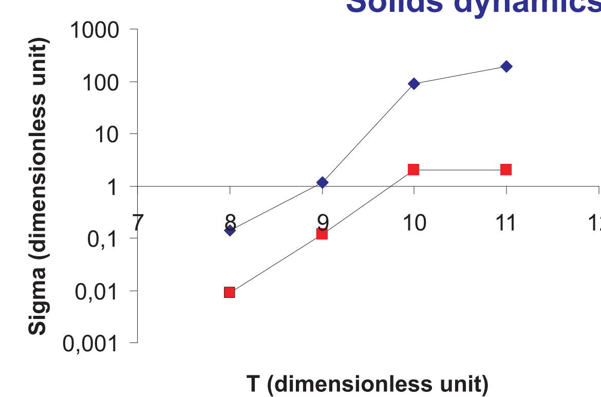
The surface density in the marked individual high-density area of gas (blue) and solids (red).
